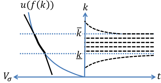
Figure 3: The limiting strategy \sigma as \varepsilon \rightarrow 0
